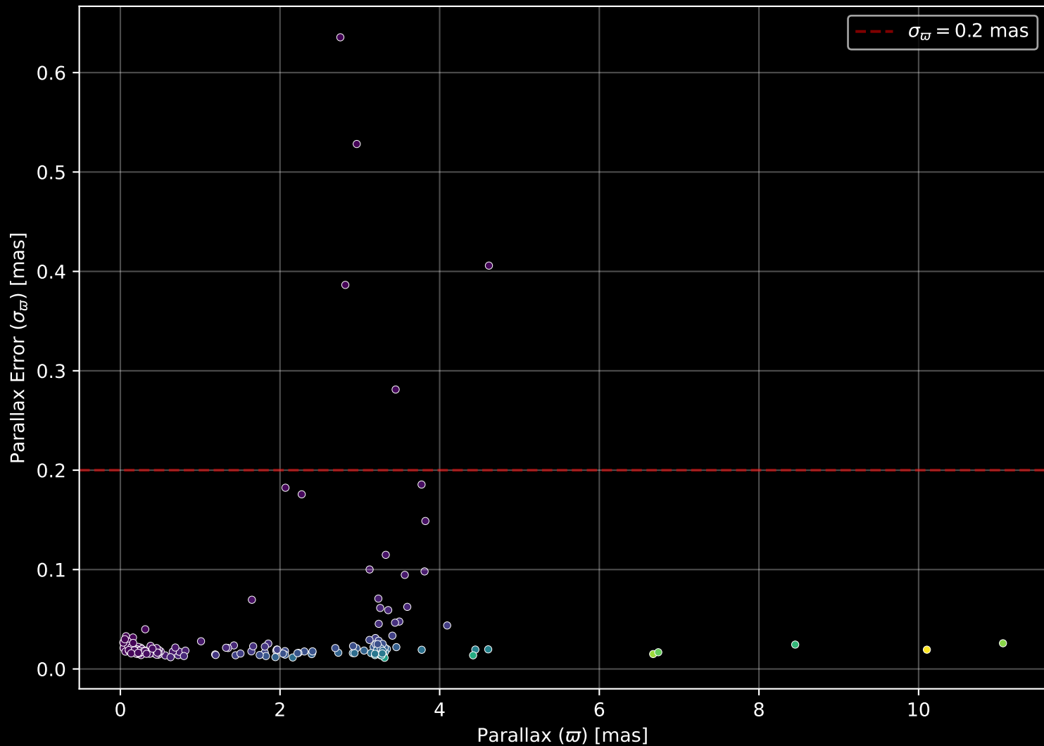
APOGEE DR17 Field: [029-12-O] Parallax Quality (n= 179)
