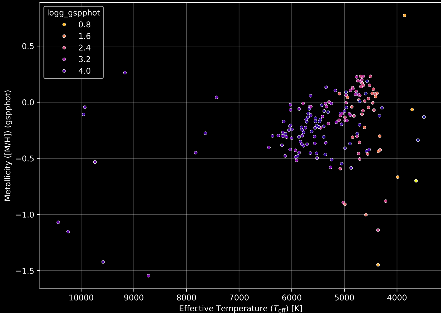
APOGEE DR17 Field: [029-12-O] Stellar Population Parameters (n= 179)
