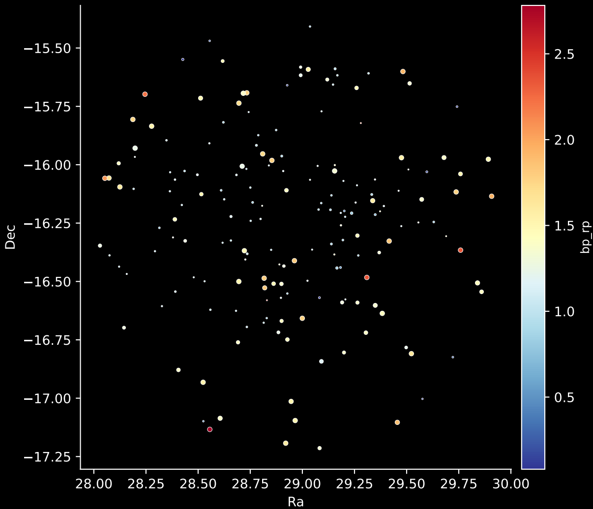
APOGEE DR17 Field: [029-12-O] Stars: 179
