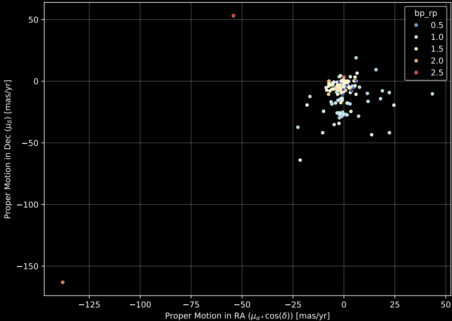
APOGEE DR17 Field: [029-12-O] Proper Motion Diagram (n= 179)
