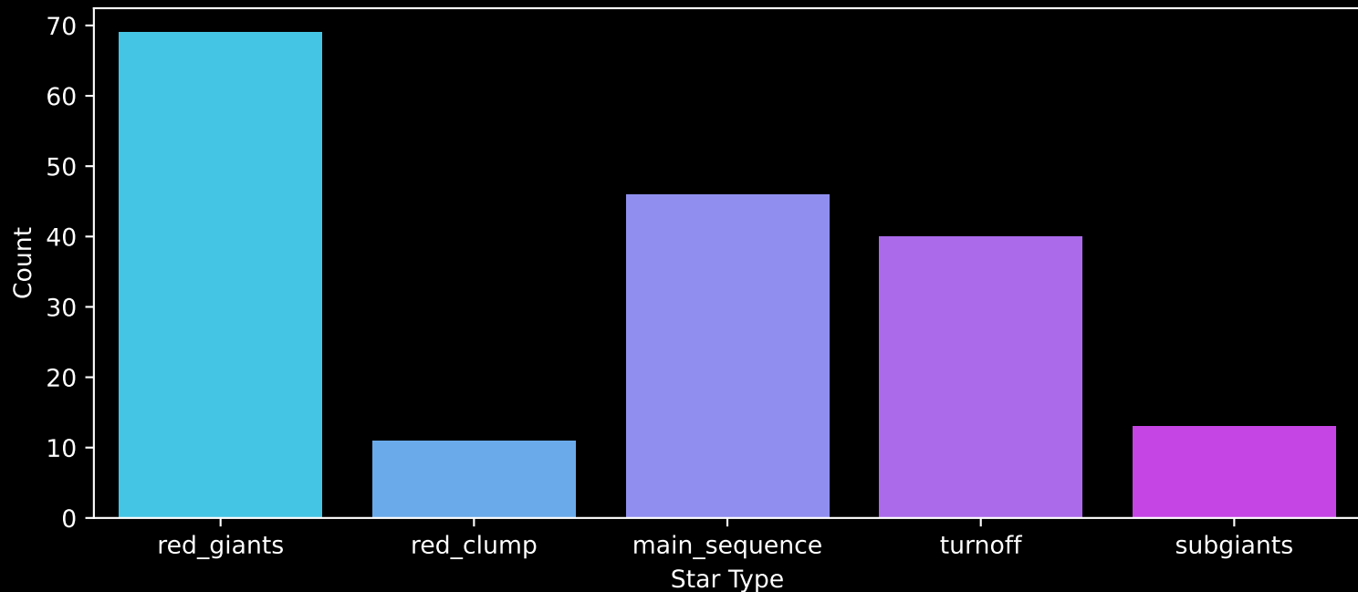
APOGEE DR17 Field: [029-12-O] Count plot of Star Type
