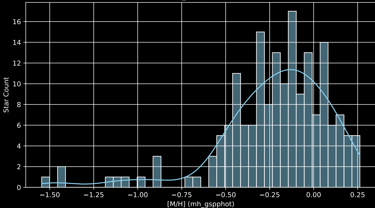
APOGEE DR17 Field: [029-12-O [M/H] (mh_gspphot) (n= 178)
