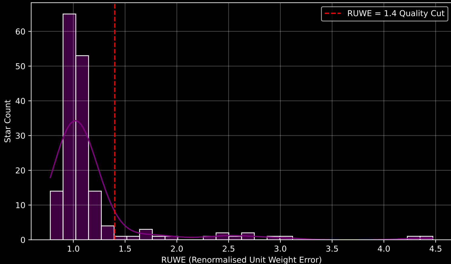
GAPOGEE DR17 Field [029-12-O] RUWE Distribution (n= 167)
