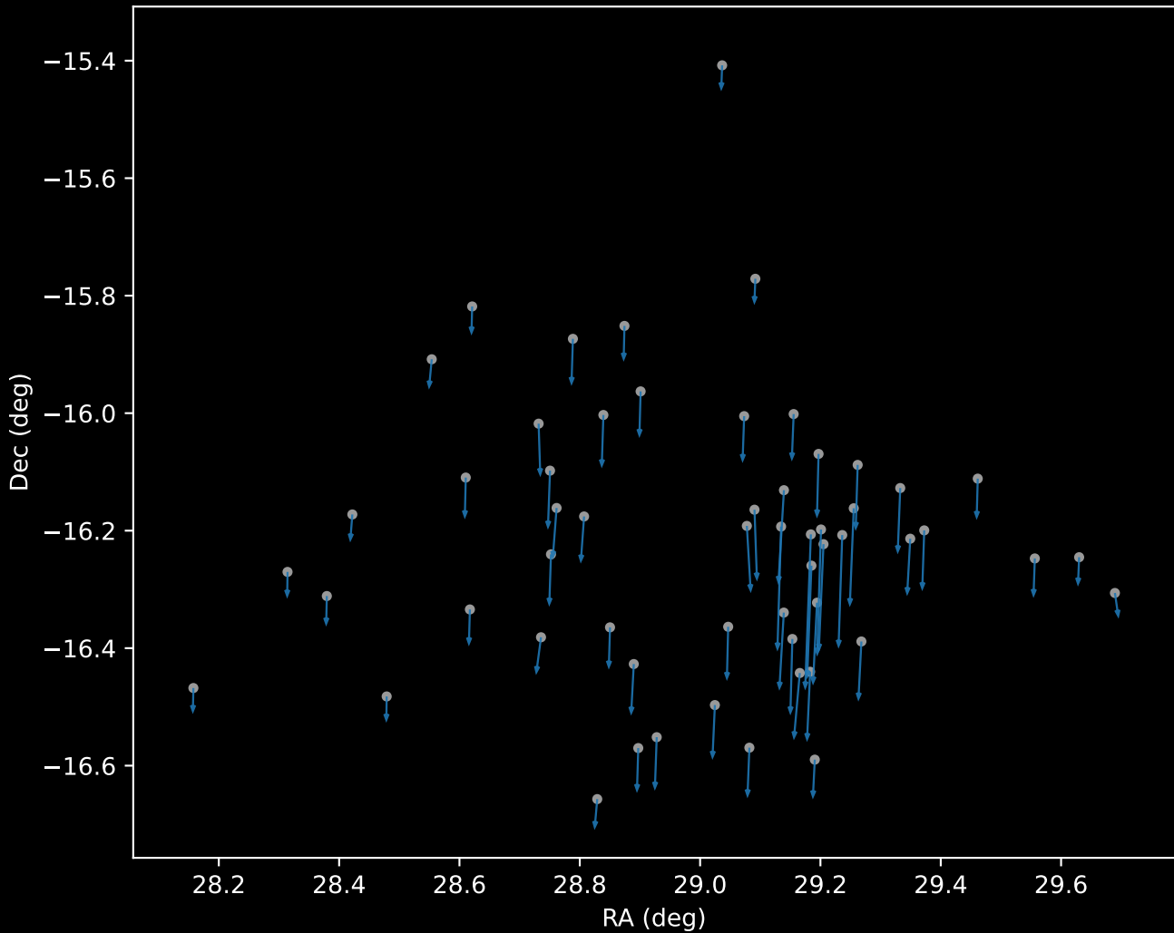
APOGEE DR17 Cluster 0 Proper Motion Vectors (n=57)
